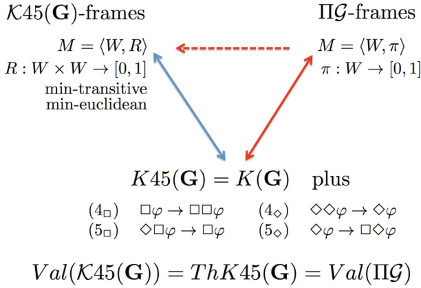
Figure 1. K45(\mathbf{G}) and its relational and possibilistic semantics
