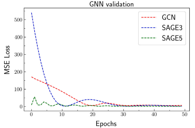
Fig. 4. Validation MSE loss after training for three of the proposed architectures: GCN, SAGE3, and SAGE5, all of them in their Medium version. The training was carried out for a fixed mask size of 0.8.
