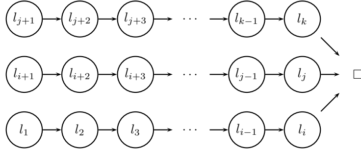
Figure 5.6: Rule 5.10 implication graph.
