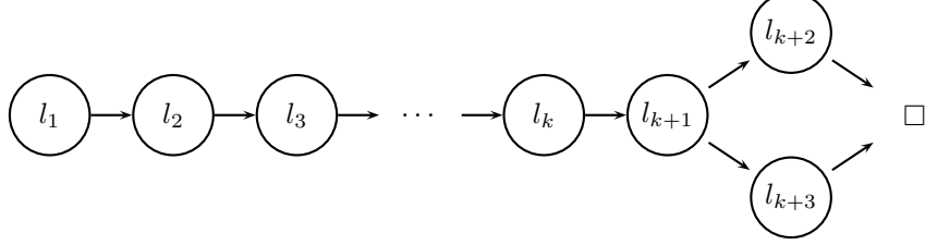
Figure 5.3: Rule 5.6 implication graph.
