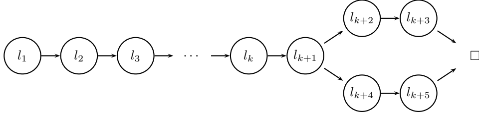
Figure 5.5: Rule 5.8 implication graph.
