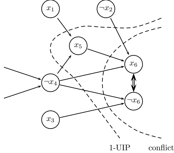
Figure 5.7: Implication graph.
