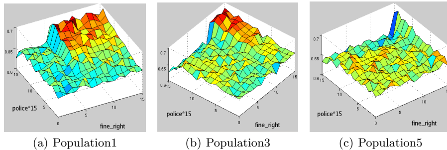
Fig. 3. Objective functions with 4 goals: col,off,expel,police. (a)Population1 ( high\_punishment = 5 ), (b)Population3 ( high\_punishment = 10 ), (c)Population5 ( high\_punishment = 14 ).
