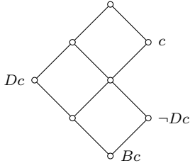
Fig. 4 Behaviour of B and D in a coatom of a residuated lattice
