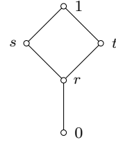
Fig. 1 A five element Gödel algebra
